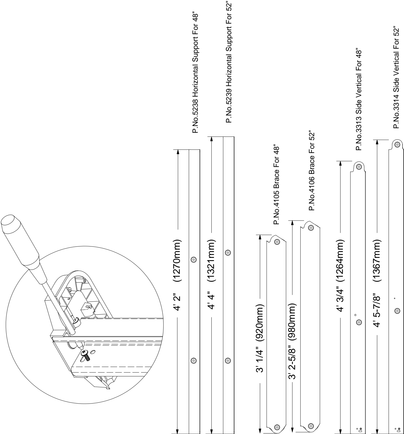
The Figure which looked at attachment of Side Upper Joint from down.
