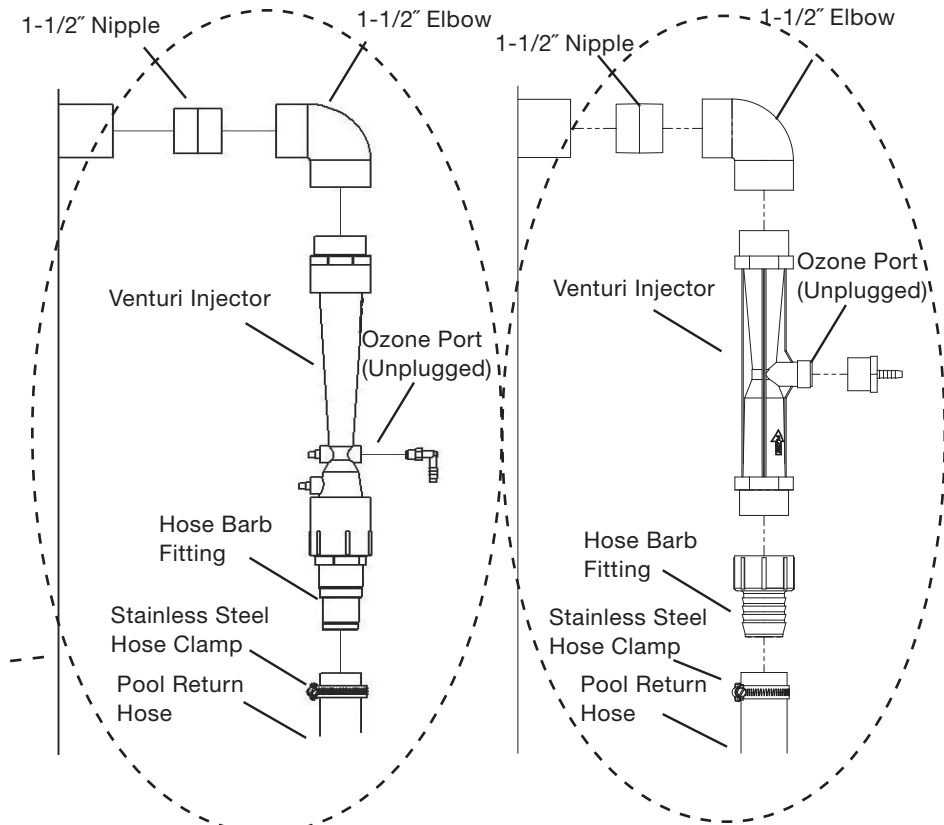
Figure 2b Mazzei Injector Assembly Exploded View
