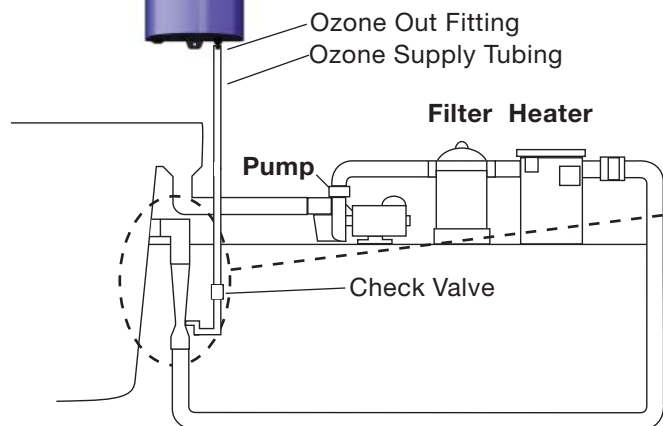
Figure 2 Installation Schematic for Injector Assembly
