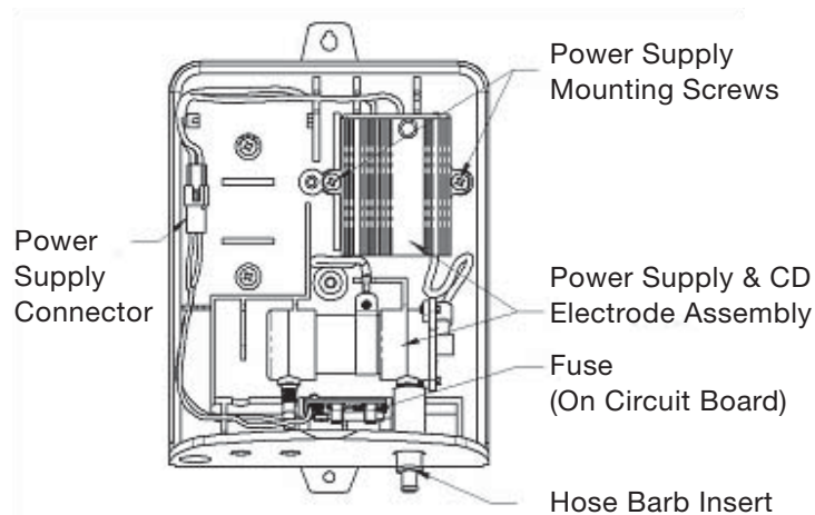
Figure 6 Internal component locations
