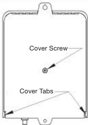
Figure 3 Cover screw and tabs
